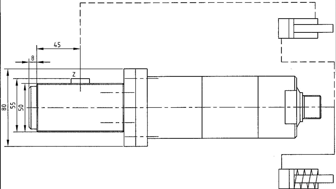
Hydraulic sketch No.: 0-208
